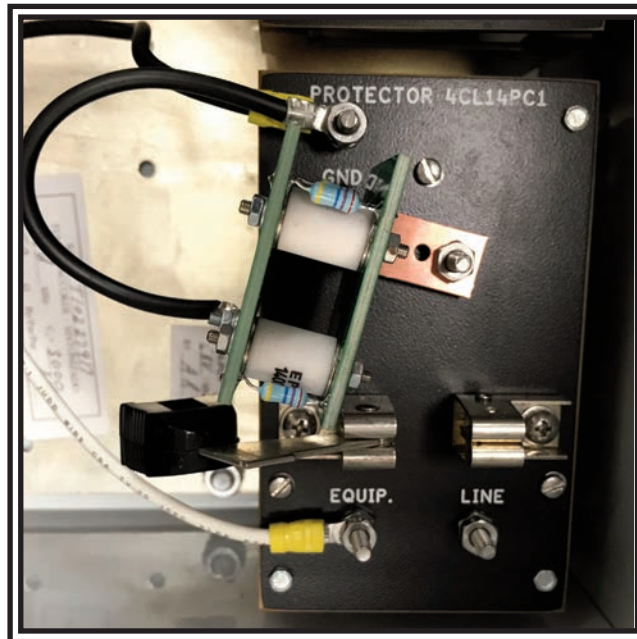
Close Up of Smart Gap in Tuner Cabinet
