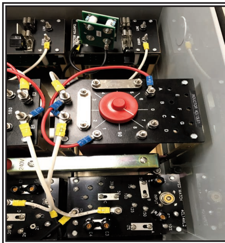
Overall View of Smart Gap in Tuner Cabinet
