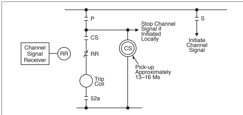
Figure 3-26b – Contact Logic (per Terminal).
