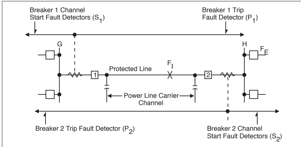
Figure 3-26a – Basic Elements for directional-comparison blocking systems.
