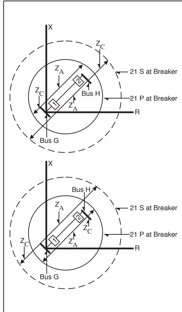
Figure 3–32. Single Phase-Comparison Blocking, Distance-Supervised Operation.
