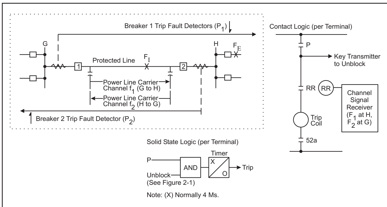
Figure 3-4. Basic Logic Diagrams for Directional Comparison Unblocking.
