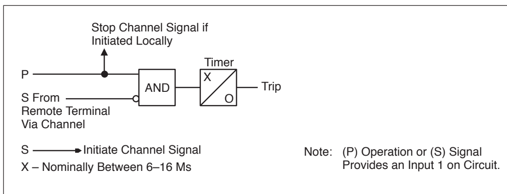
Figure 3-26c – Solid State Logic (per Terminal).
