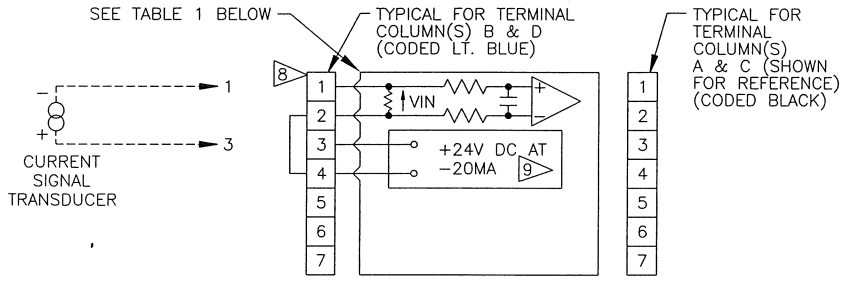
SIGNAL INPUT WIRING DIAGRAM
